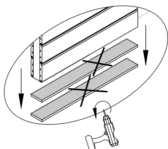
INSULATED FLOOR WITH TONGUE AND GROOVE BOARD
