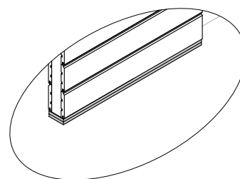
COLD FLOOR WITH BOARD
